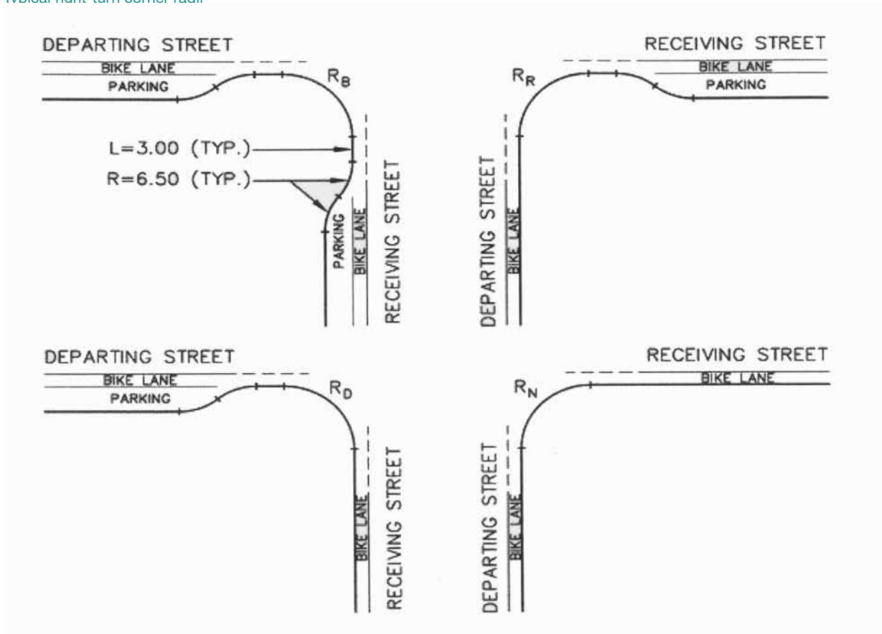
Figure 3.7-8: Typical right-turn corner radii
