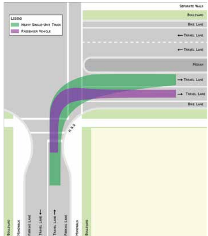
Figure 3.7-7: Auto turning templates
