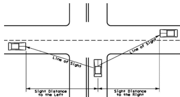
Figure 3.1-15: Intersection sight distance
