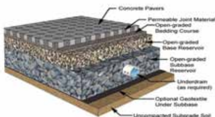
Figure 3.6-7: Typical permeable pavement details (Smith 2009)
