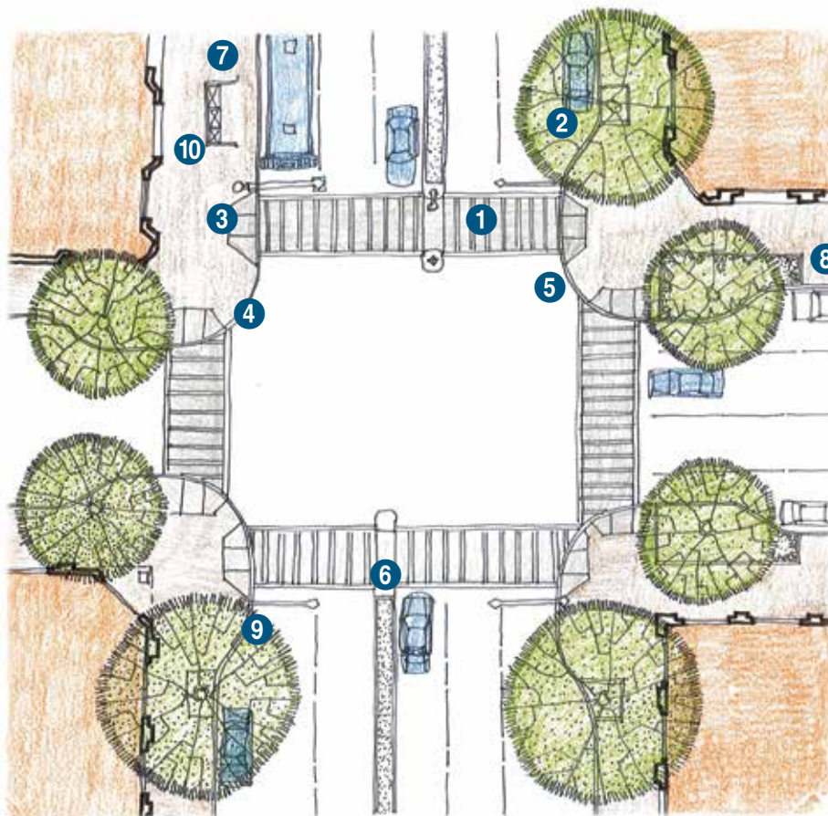
Figure 3.7-12: Elements of a good intersection
