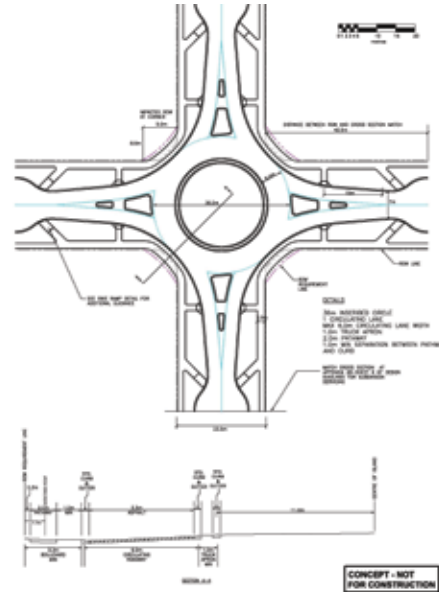
Figure D.3-1: Roundabout – undivided primary collector
