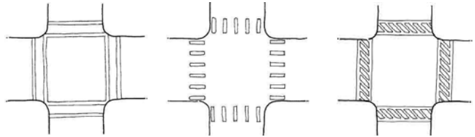
Figure 3.2-5: Crosswalk pavement markings (FWHA, Sidewalk Design Guidelines )
