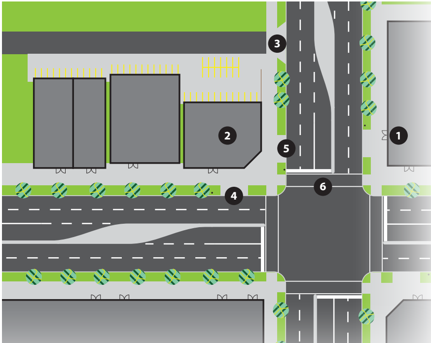
Figure 3.4-11: Transit stop design considerations (continued)
