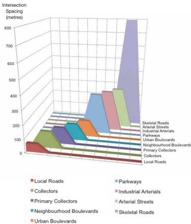
Figure 3.7-1: Minimum Intersection Spacing
