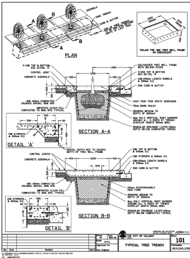
Figure 3.6-9: Tree trench specifications
