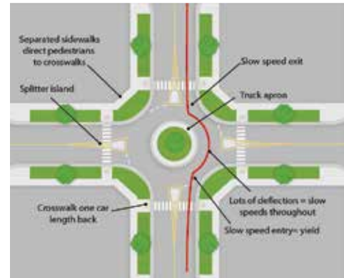
Figure 3.7-11: Roundabout
