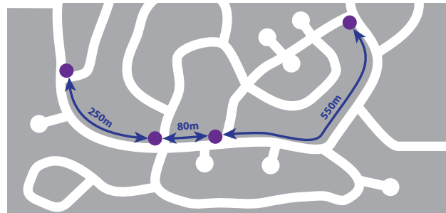
Figure 3.4-13: Irregularly spaced intersections and restricted pedestrian access leads to irregularly spaced bus zones. This can be difficult for customers to access the service and negatively impacts the walkability to and from transit service.
