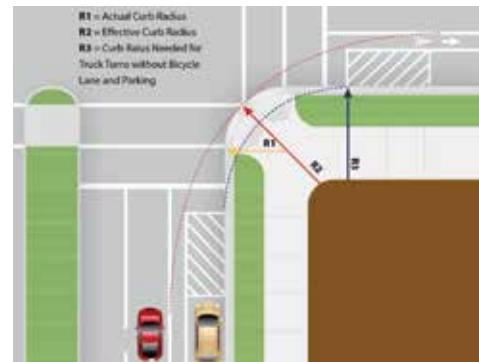
Figure 3.7-5: Corner radius
