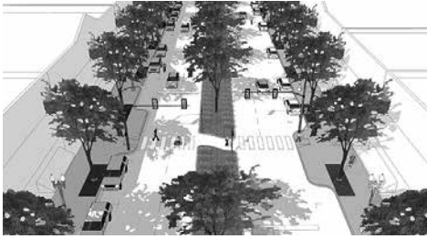
Figure 3.2-11: Angled median crossing (Credit: ite.org)
