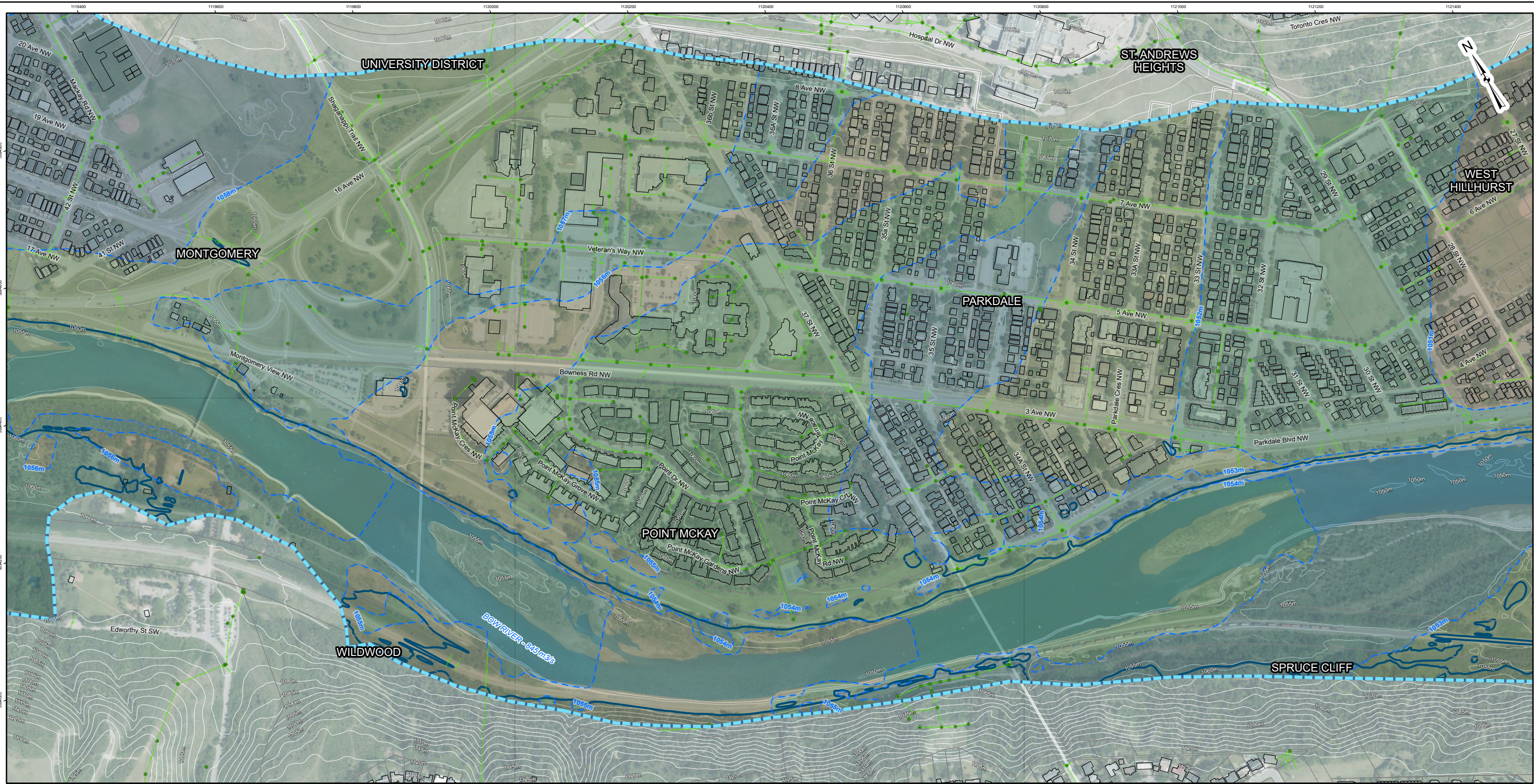
FIGURE 2.3 GROUNDWATER ELEVATION SIMULATION (CALIBRATED MODEL) 1 IN 10 YEAR FLOOD 4 - POINT MCKAY
