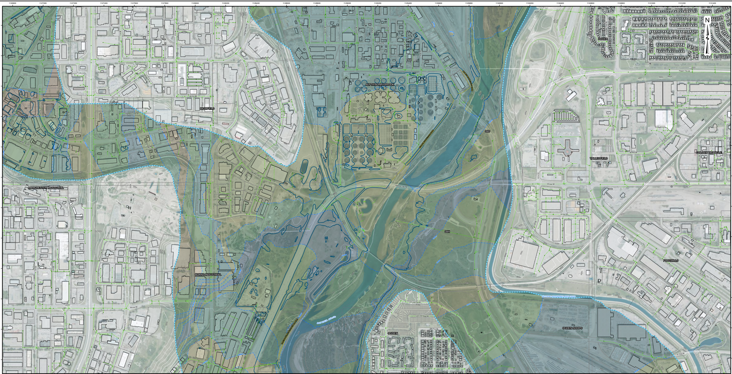
FIGURE 2.3 GROUNDWATER ELEVATION SIMULATION (CALIBRATED MODEL) 1 IN 10 YEAR FLOOD 13 - BONNYBROOK
