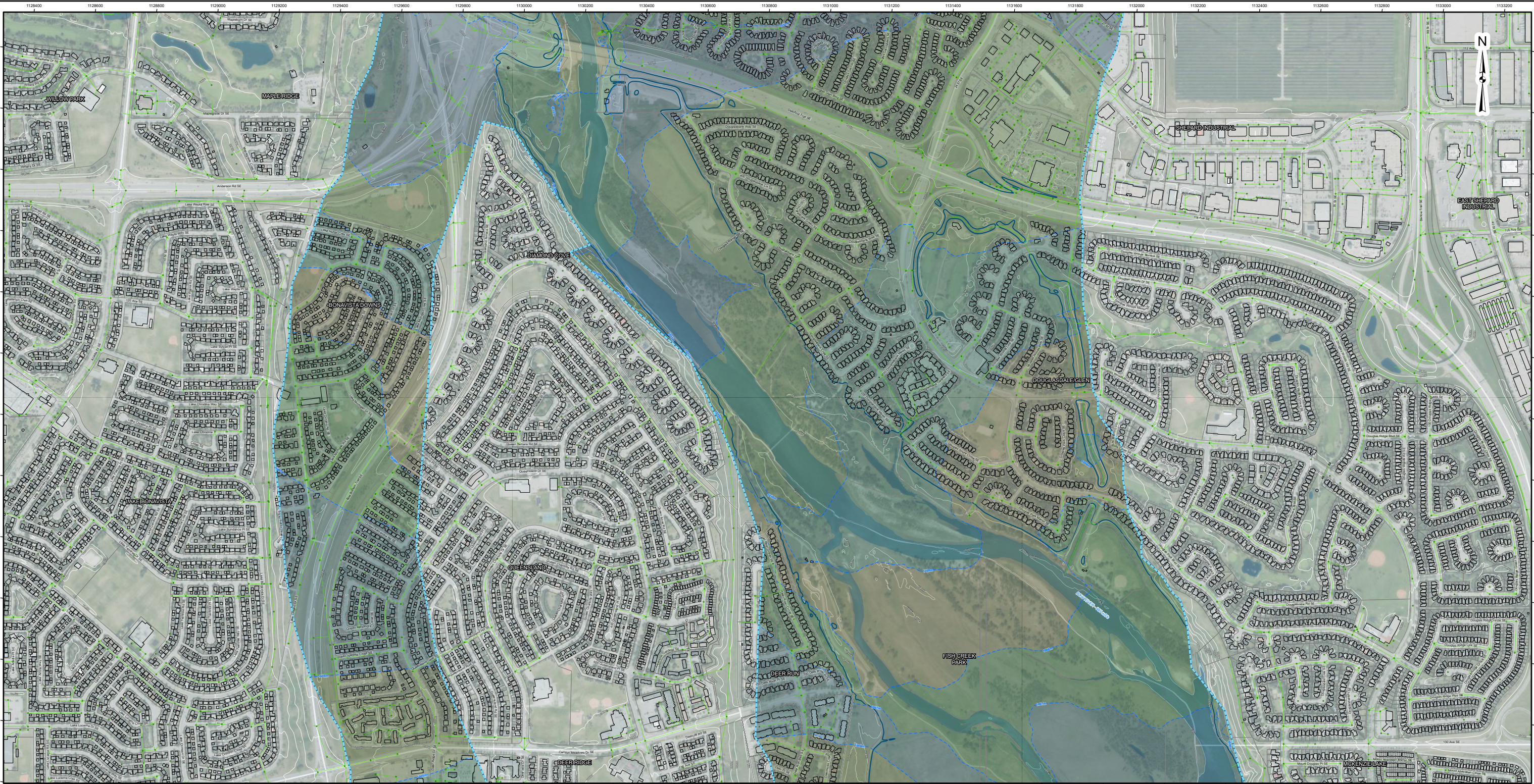
FIGURE 2.3 GROUNDWATER ELEVATION SIMULATION (CALIBRATED MODEL) 1 IN 10 YEAR FLOOD 16 - DOUGLASDALE
