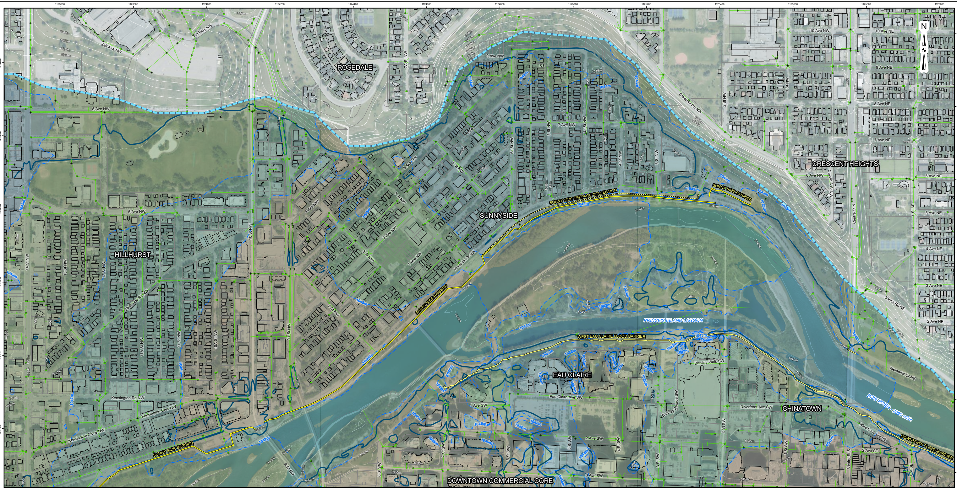
FIGURE 2.4 GROUNDWATER ELEVATION SIMULATION (CALIBRATED MODEL) 1 IN 20 YEAR FLOOD 6 - SUNNYSIDE
