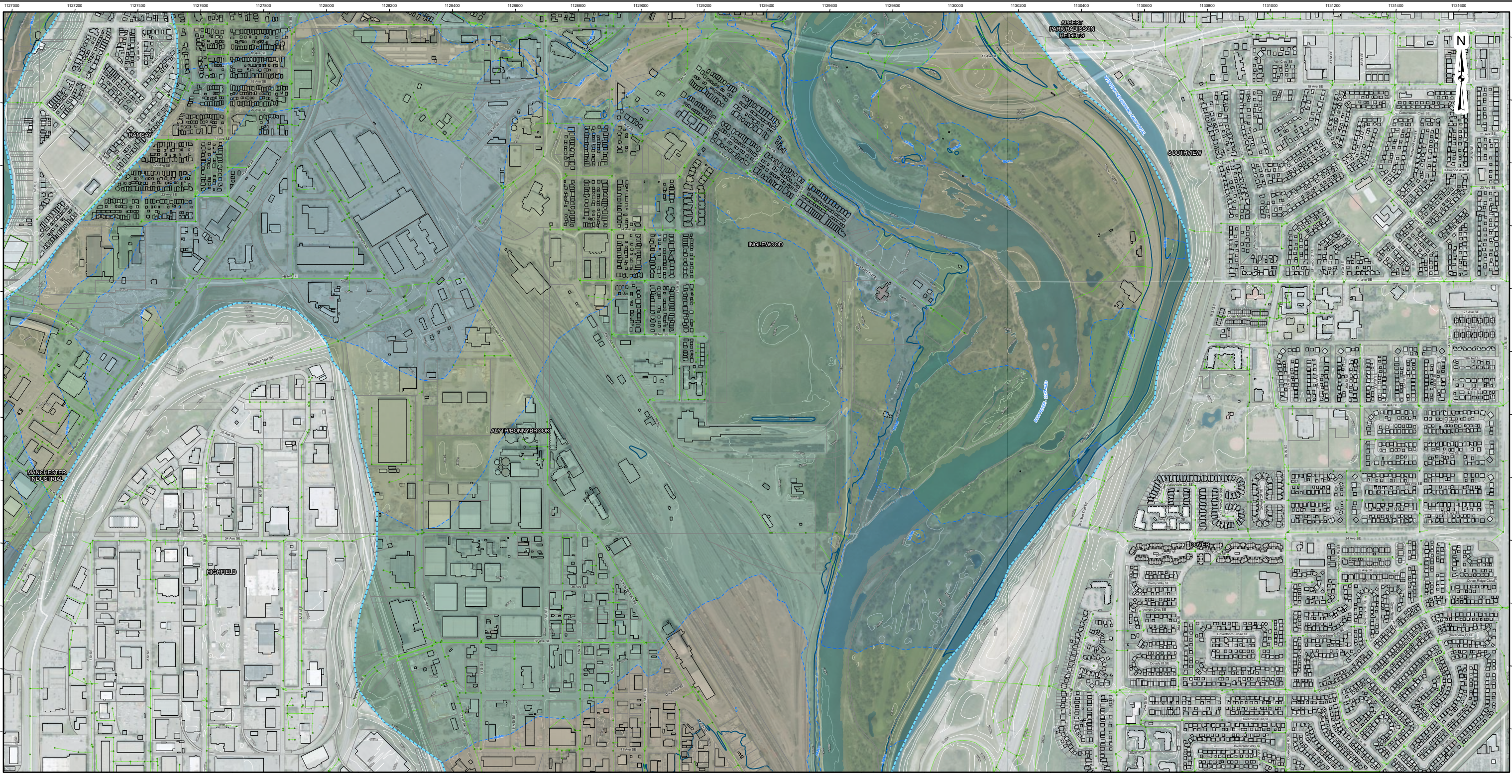
FIGURE 2.4 GROUNDWATER ELEVATION SIMULATION (CALIBRATED MODEL) 1 IN 20 YEAR FLOOD 12 - INGLEWOOD - BONNYBROOK
