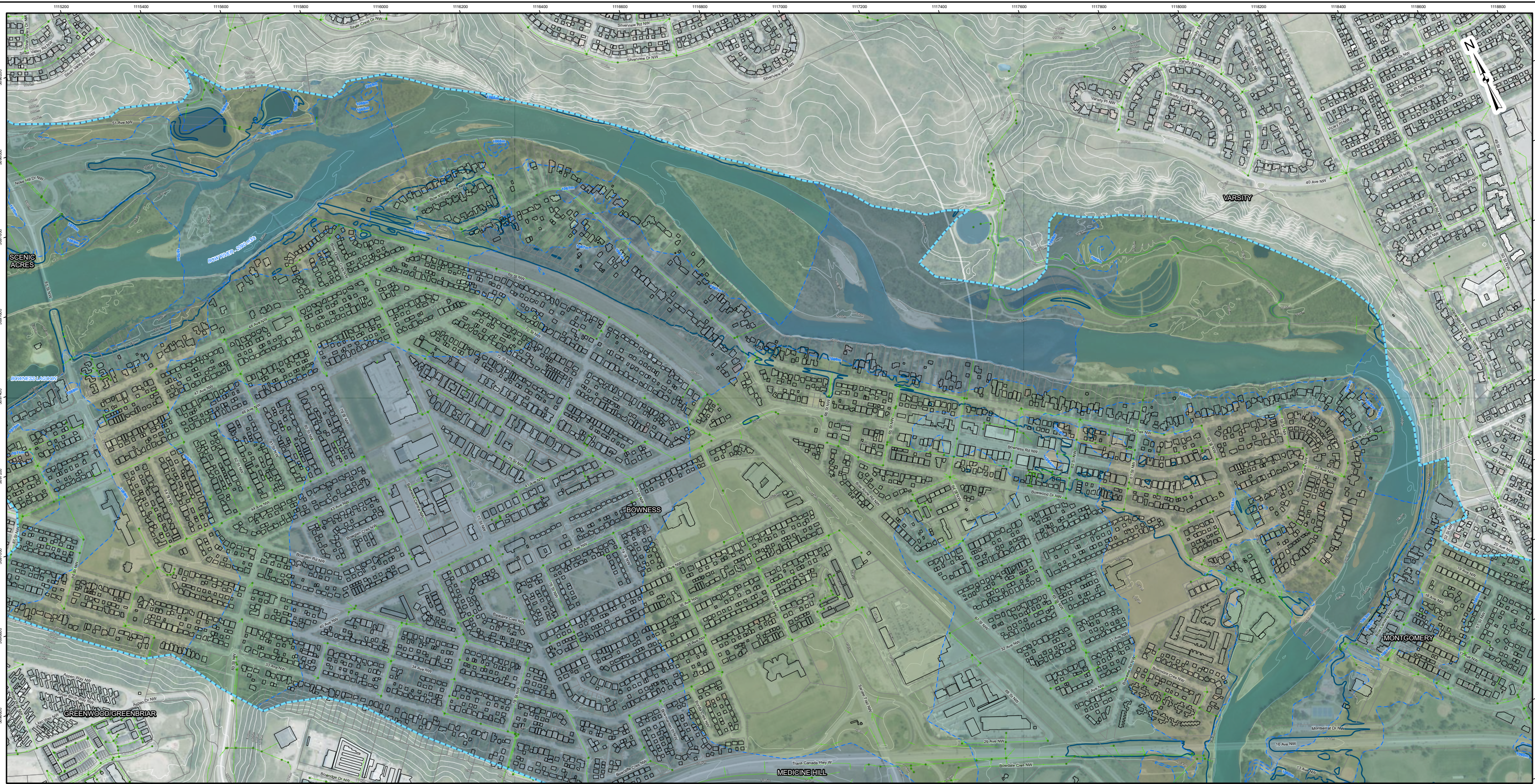
FIGURE 2.4 GROUNDWATER ELEVATION SIMULATION (CALIBRATED MODEL) 1 IN 20 YEAR FLOOD 2 - BOWNESS
