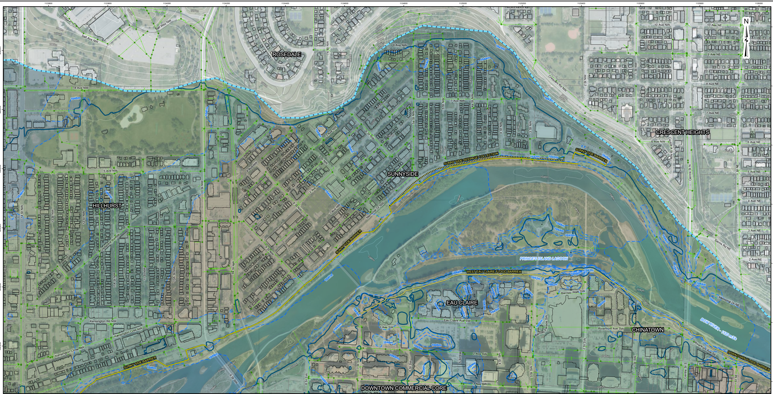
FIGURE 2.5 GROUNDWATER ELEVATION SIMULATION (CALIBRATED MODEL) 1 IN 50 YEAR FLOOD 6 - SUNNYSIDE
