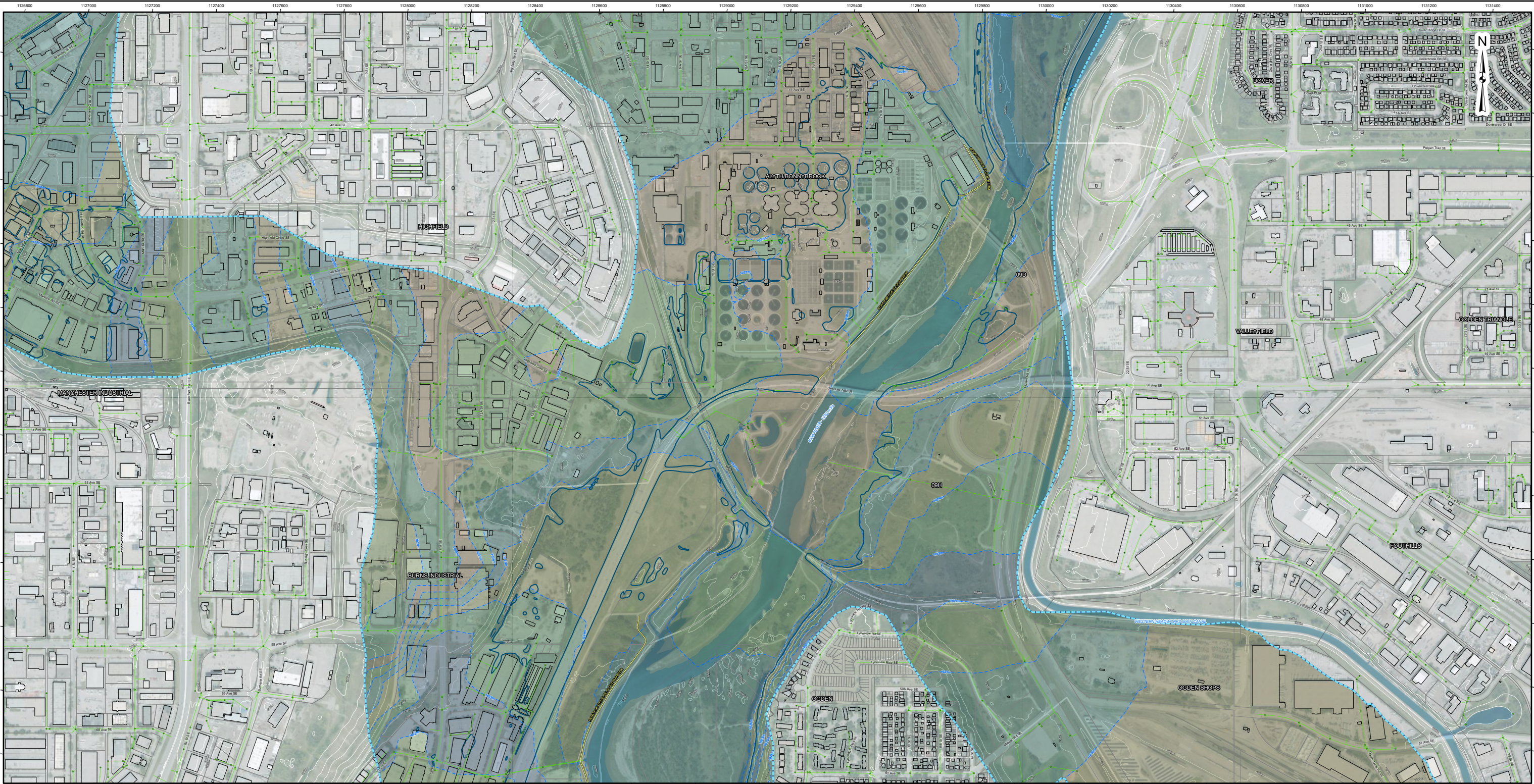
FIGURE 2.5 GROUNDWATER ELEVATION SIMULATION (CALIBRATED MODEL) 1 IN 50 YEAR FLOOD 13 - BONNYBROOK
