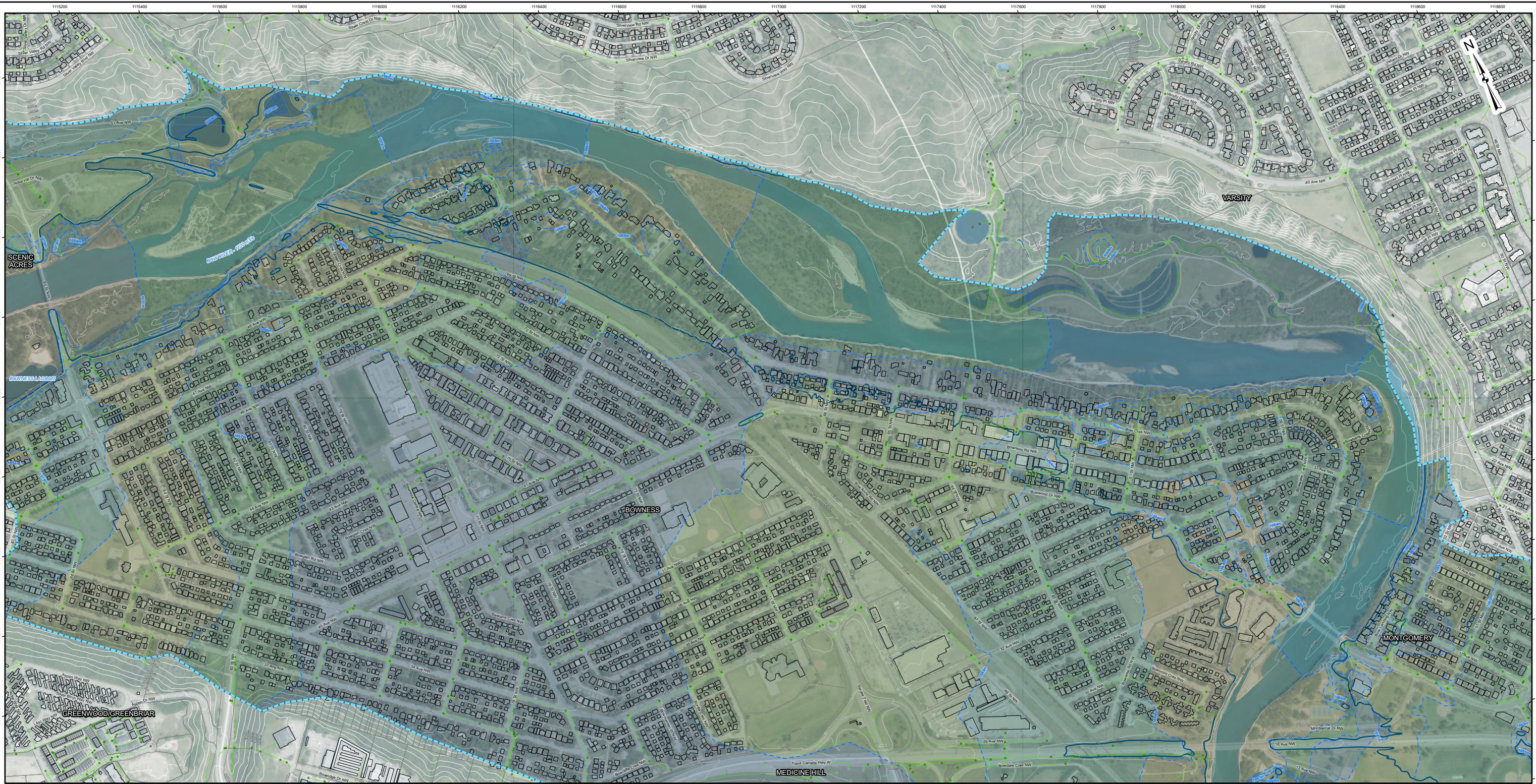
FIGURE 2.5 GROUNDWATER ELEVATION SIMULATION (CALIBRATED MODEL) 1 IN 50 YEAR FLOOD 2 - BOWNESS
