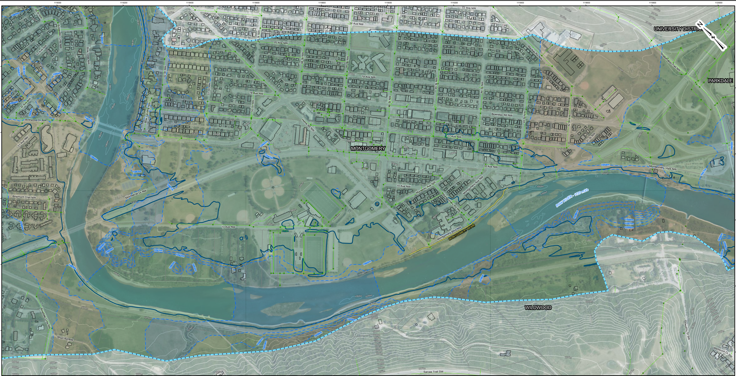
FIGURE 2.5 GROUNDWATER ELEVATION SIMULATION (CALIBRATED MODEL) 1 IN 50 YEAR FLOOD 3 - MONTGOMERY
