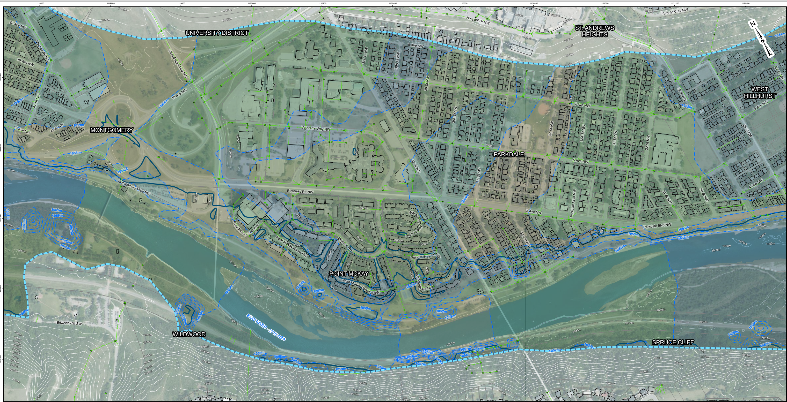
FIGURE 2.7 GROUNDWATER ELEVATION SIMULATION (CALIBRATED MODEL) 1 IN 200 YEAR FLOOD 4 - POINT MCKAY
