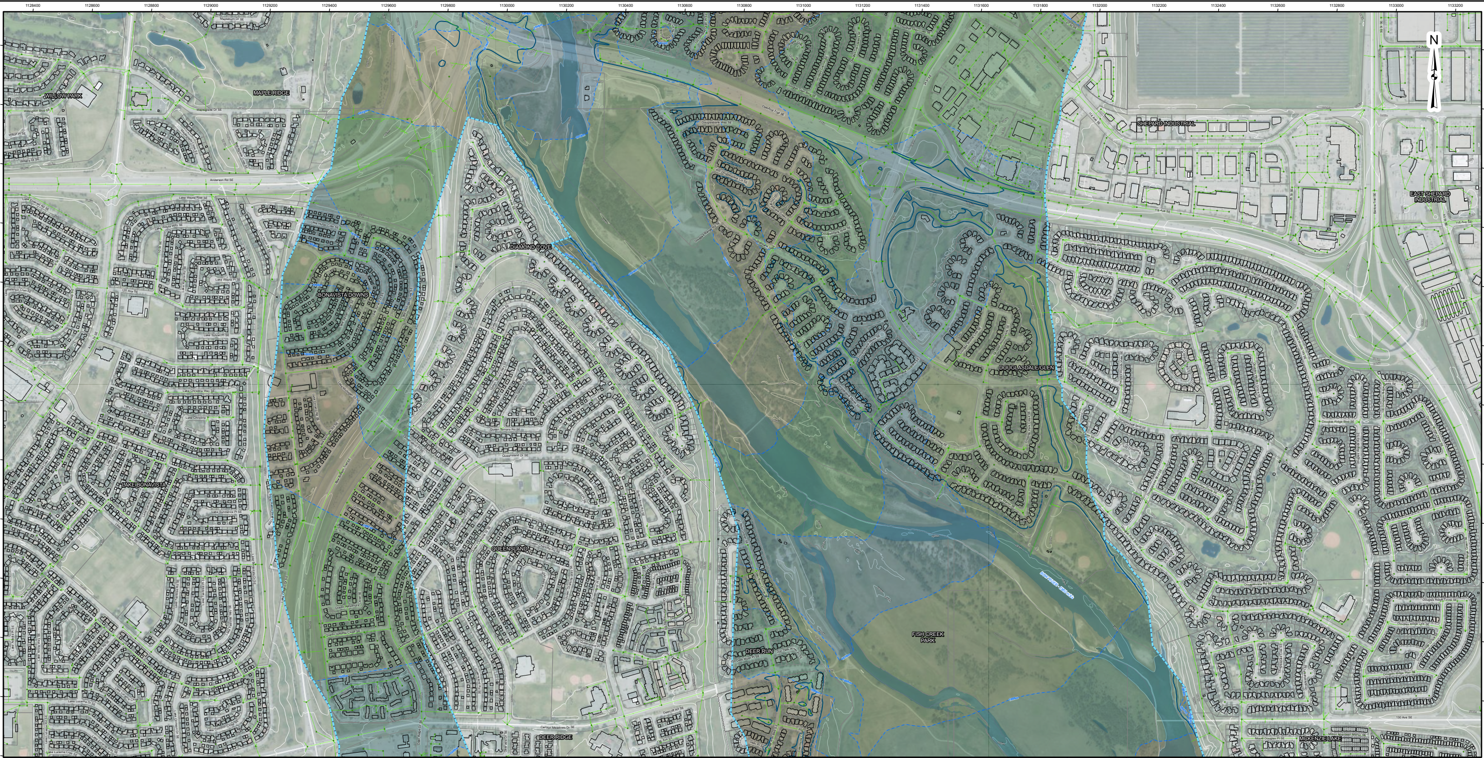
FIGURE 2.7 GROUNDWATER ELEVATION SIMULATION (CALIBRATED MODEL) 1 IN 200 YEAR FLOOD 16 - DOUGLASDALE
