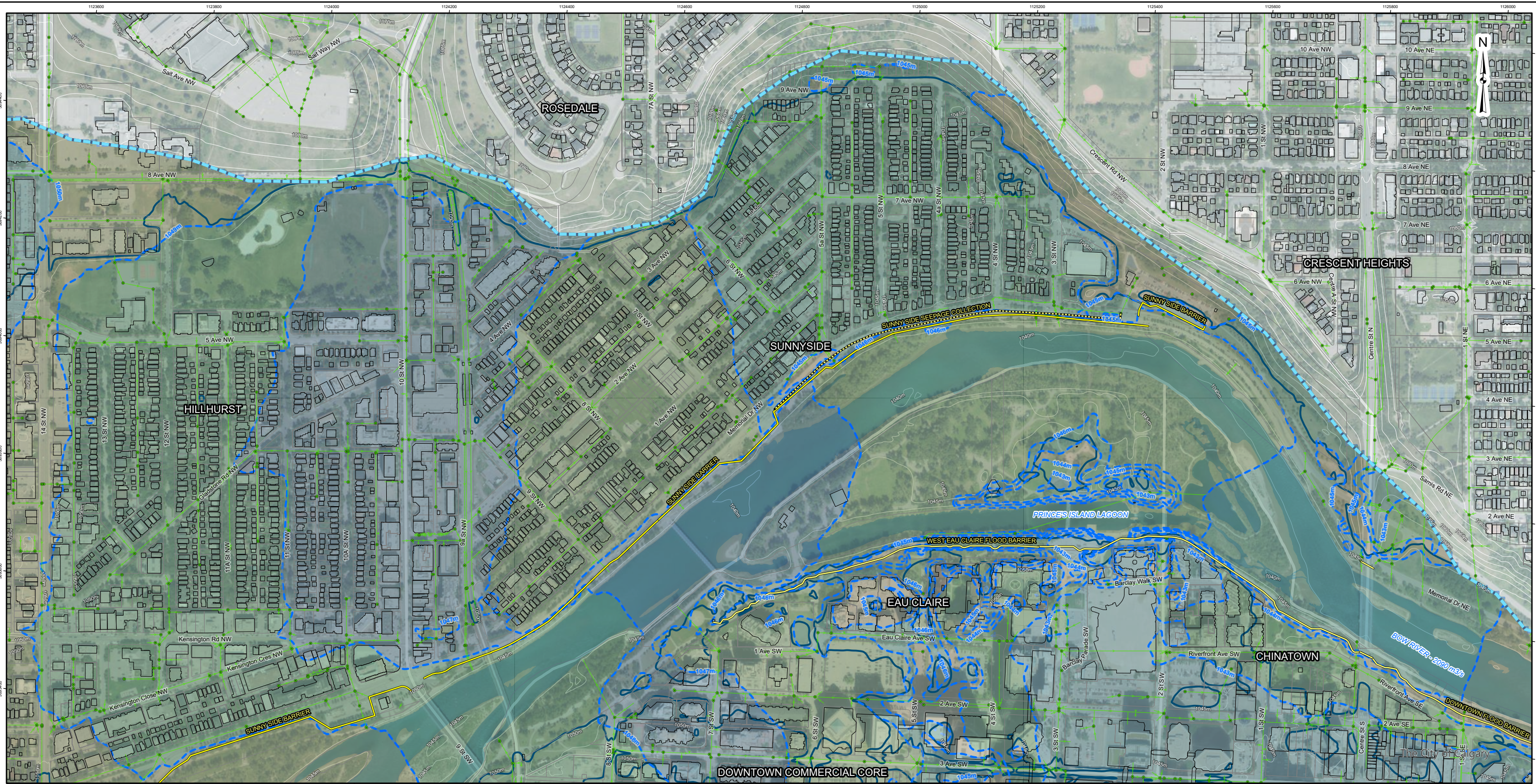
FIGURE 2.8 GROUNDWATER ELEVATION REPRESENTATION (P90) 1 IN 100 YEAR FLOOD 6 - SUNNYSIDE
