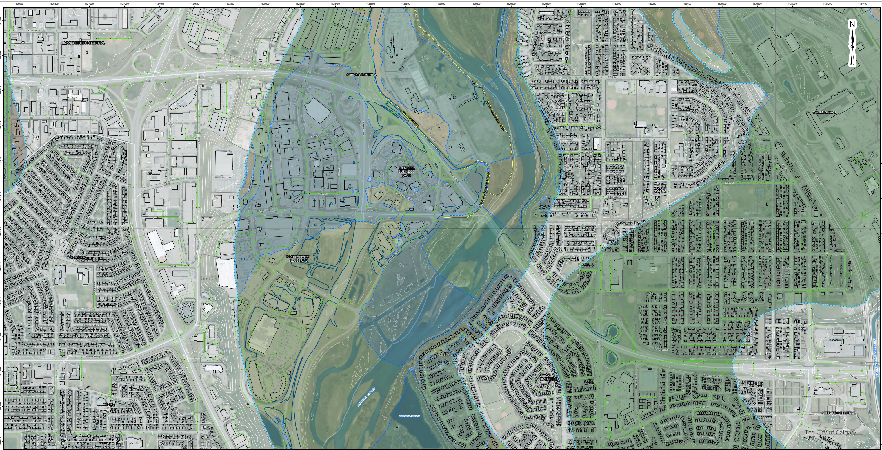
FIGURE 2.8 GROUNDWATER ELEVATION REPRESENTATION (P90) 1 IN 100 YEAR FLOOD 14 - DEERFOOT MEADOWS
