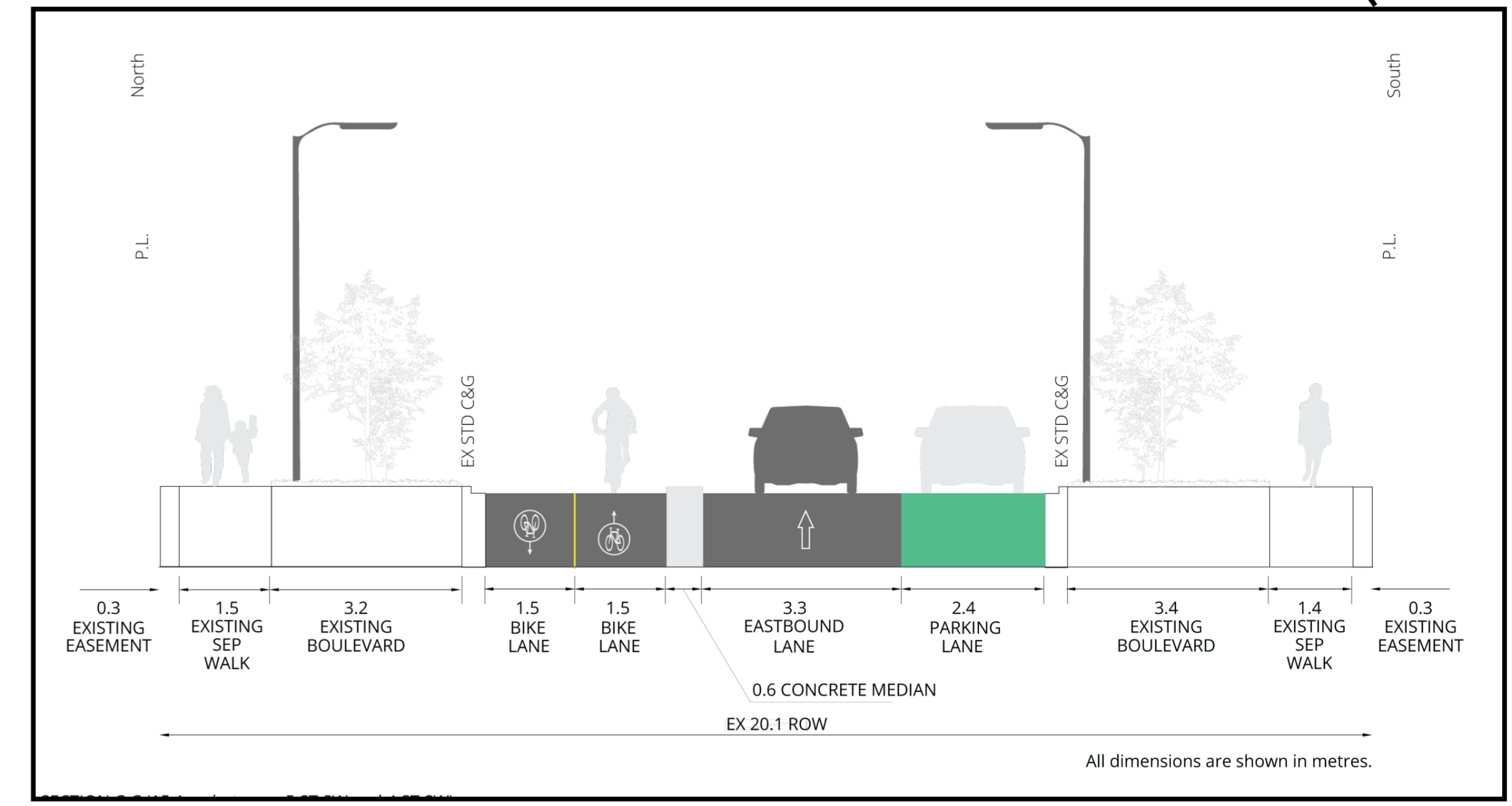
Cross Section C-C, 15 Avenue East of 5 Street SW
